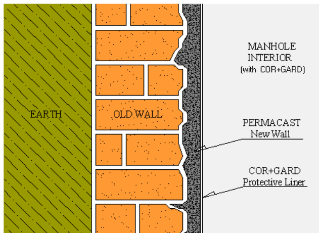
Typical cross section of PERMACAST® shell
