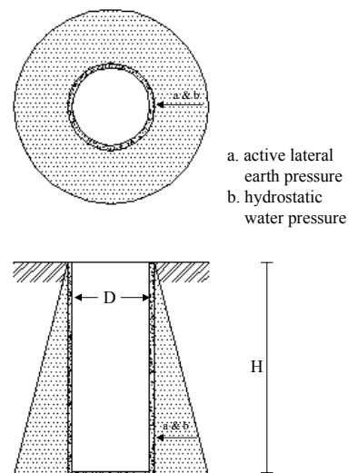
Figure 4. Triangular distribution of lateral loads acting on manhole
