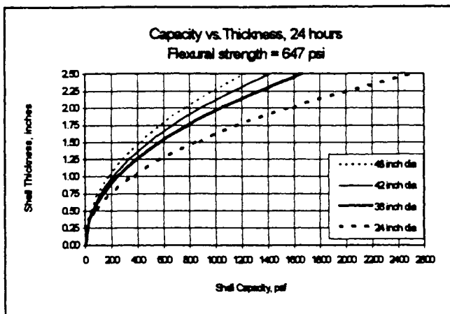
Figure 1. Moment load capacity of shells, 24 hour test
