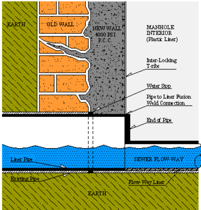
Typical cross section of PERMAFORM® manhole
