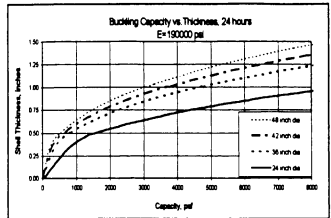
Figure 2. Buckling capacity, 24 hour test
