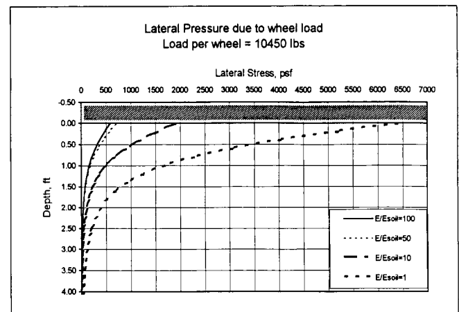
Figure 3. Lateral stresses due to wheel load
